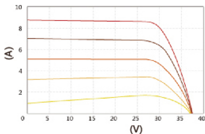
I-V Curve ( JY270P6-Ab-5 )
